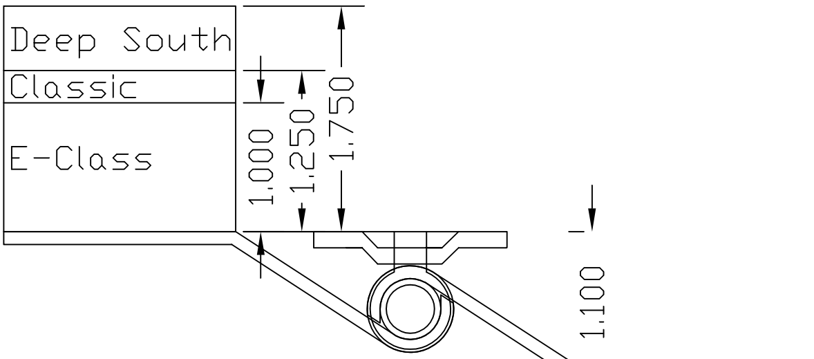
1/2" Pintle, 1/2" Strap
