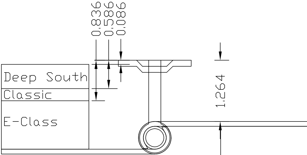
1 1/2" Pintle, Flat Strap
