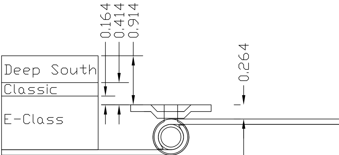
1/2" Pintle, Flat Strap
