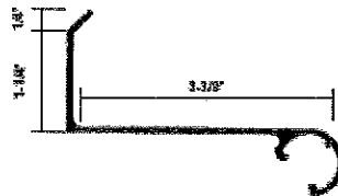
3¾" Female Hinge
